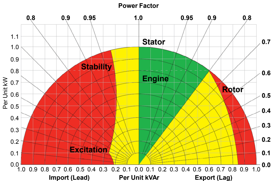
Figure 7 Sample of a generator capability curve showing acceptable operating conditions for load and power factor
