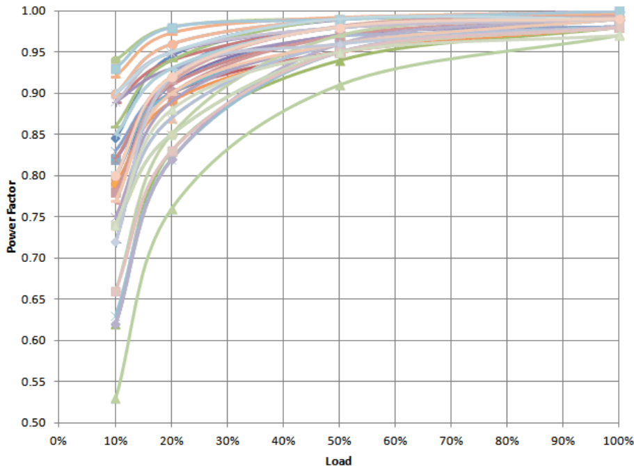
Power Factor vs. Load (Gold Only)
